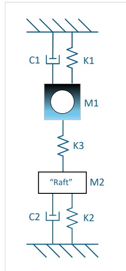
Figure 6: Two-stage washing machine mount system.
